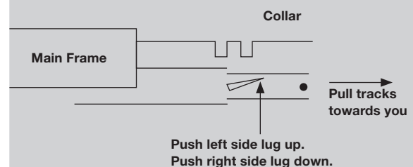
FIGURE 1 – TRACK REMOVAL (LEFT SIDE)
